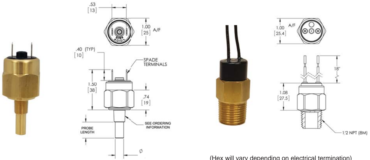
(Hex will vary depending on electrical termination)
