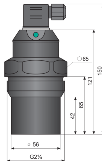
Measuring Range M1 (0.40 ... 10 meters)
