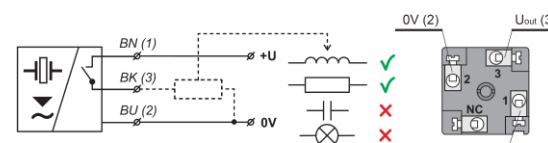
Connection diagram of the P421 sensor with the PNP switching transistor with an open collector output
