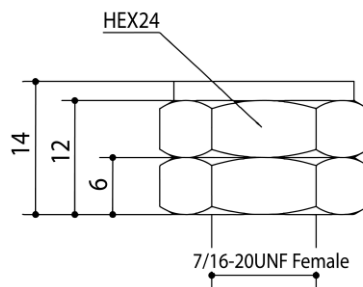
7/16"-20UNF female SAE J512 with valve opener
