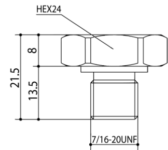
7/16"-20UNF-2A male SAE J1926-2
