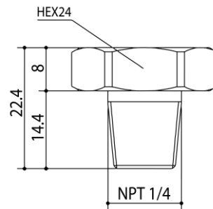
1/4" NPT male
