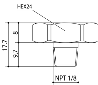
1/8" NPT male
