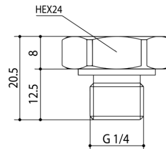
G1/4" male
