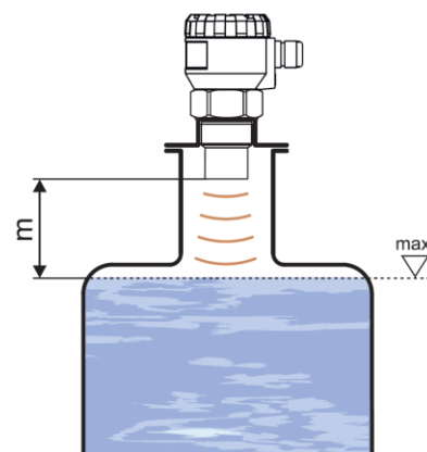
Maximum level distance from P103
