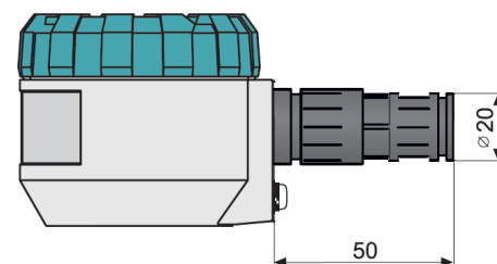
P103 with protective connector
