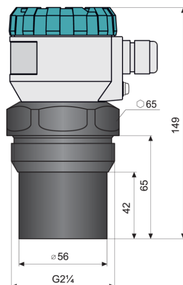
Measuring Distance M3 (0.20 ... 6.0 meters)
