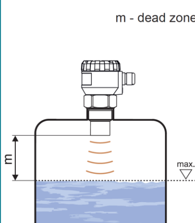
Maximum level distance from P103
