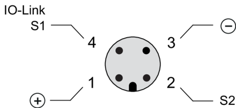
Transmitter IO-Link (Type series PA2530)
