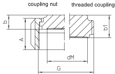
sanitary connection per IDF-Norm
