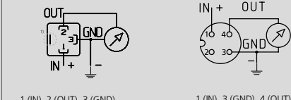
1 (IN) 2 (OUT) 3 (GND) 1 (IN) 3 (GND) 4 (OUT)
