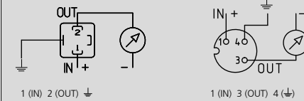
1 (IN) 2 (OUT) 1 (IN) 3 (OUT) 4 (GND)
