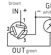
1 (IN) 2 (OUT) 3 (GND)
