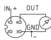
1 (IN) 4 (OUT) 3 (GND)
